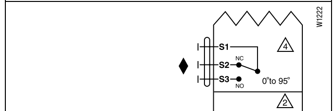
Auxiliary switch of TFB24-MFT(-S), TFX24-MFT(-S)
