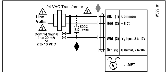
VDC/ 4-20 mA
