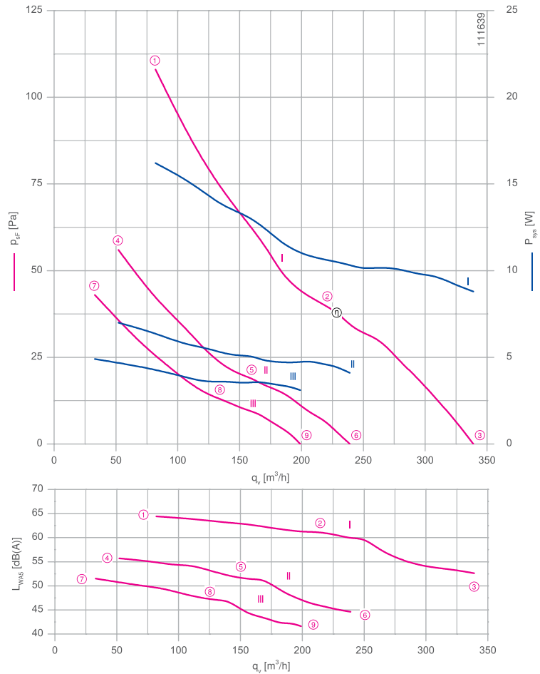
Measured with inlet ring, without guard grille in installation typet A according to ISO 5801
