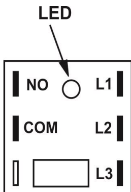
THREE-PHASE MONITOR
