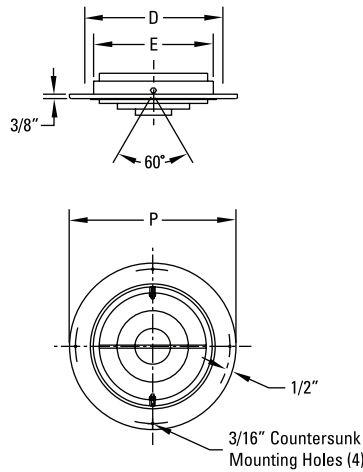
ANC-RP Dimensions in Inches
