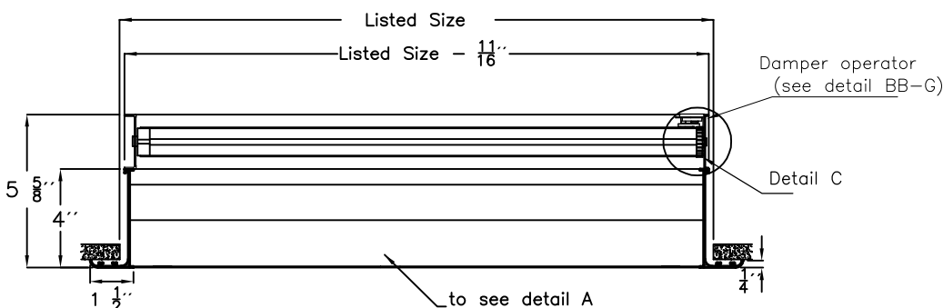
SECTION C-C
