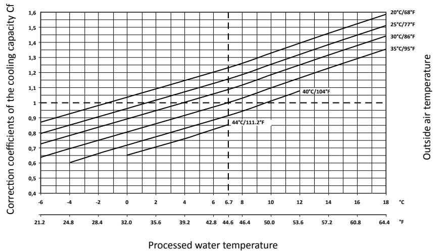
CORRECTION COEFFICIENTS OF THE COOLING CAPACITY
